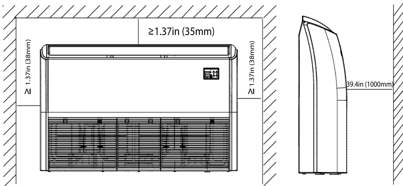
Fig. 7 — Clearance for 18K-24K
